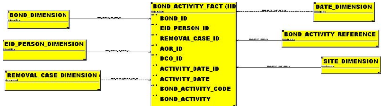
Figure 10. Bond Activity Dimensional Model
