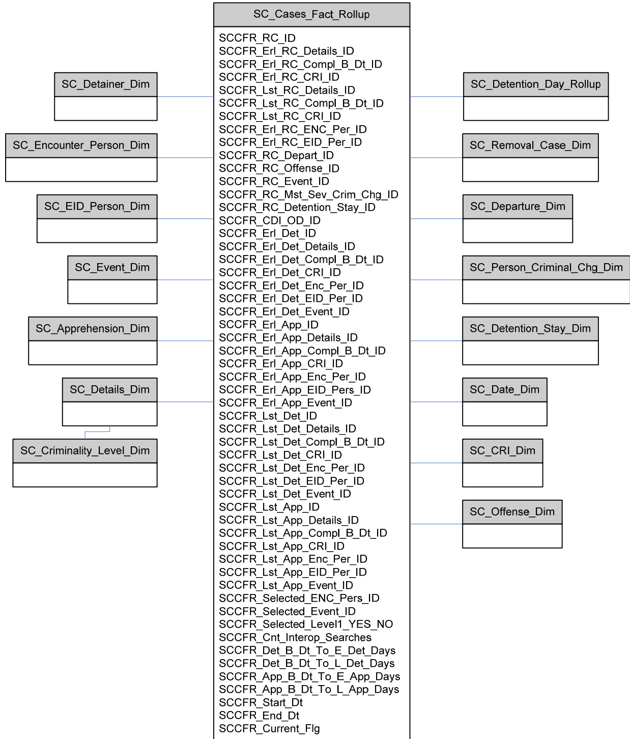
Figure 14. Secure Communities Cases Rollup Dimensional Model
