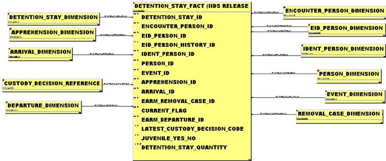
Figure 6. Detention Stay Dimensional Model
