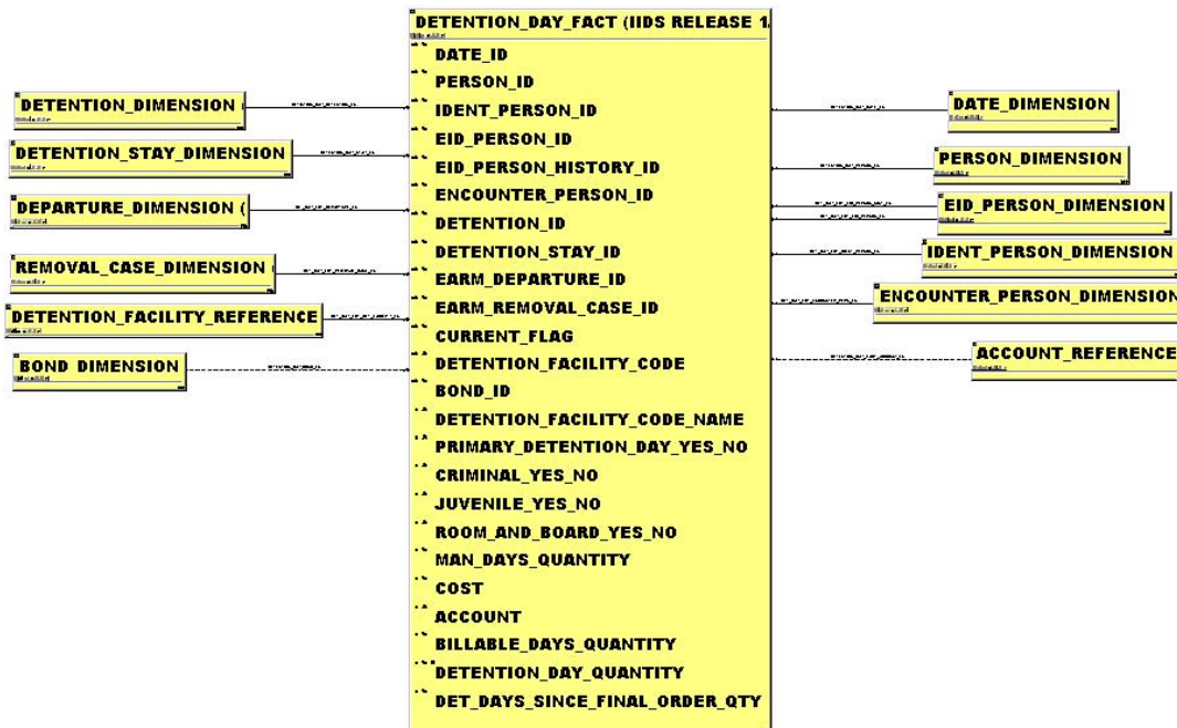
Figure 5. Detention Day Dimensional Model
