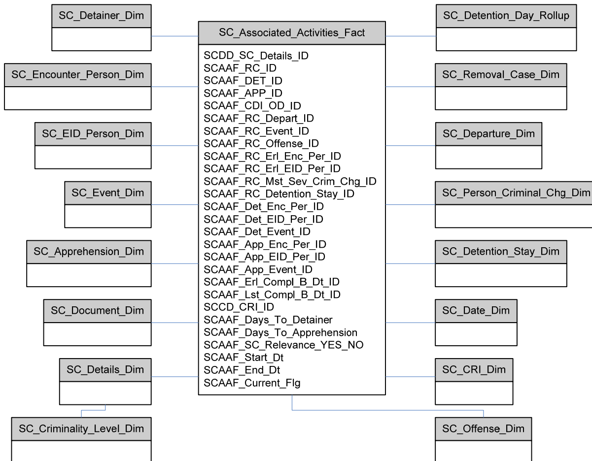
Figure 13. Secure Communities Associated Activities Dimensional Model
