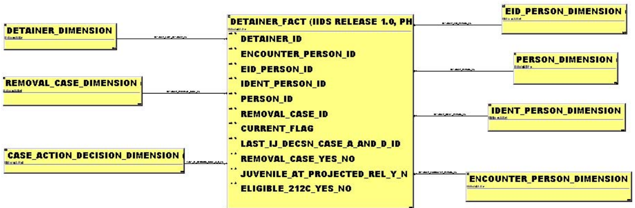
Figure 8. Detainer Dimensional Model
