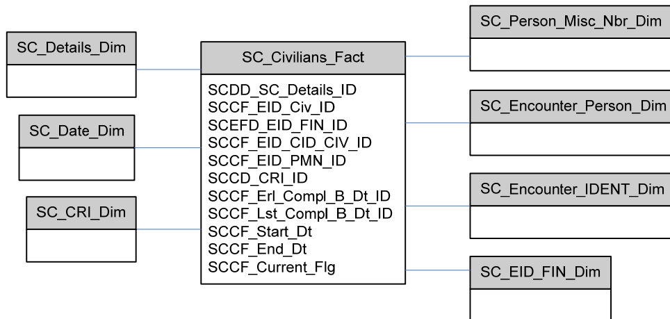
Figure 12. Secure Communities Civilians Dimensional Model
