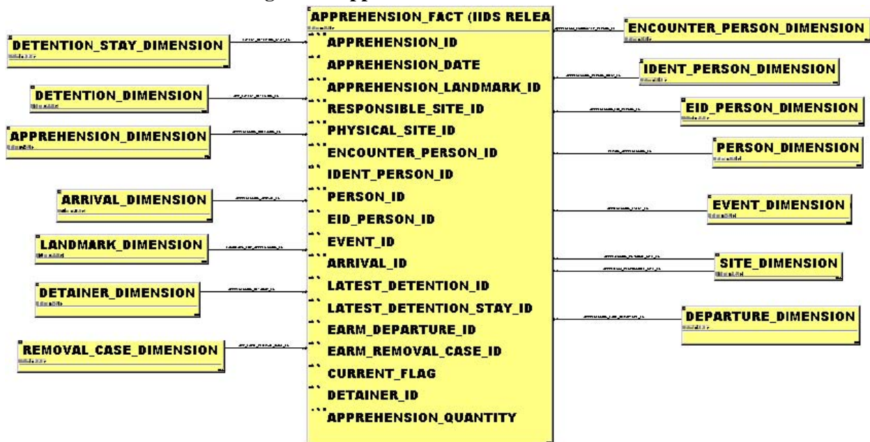
Figure 3. Apprehension Dimensional Model
