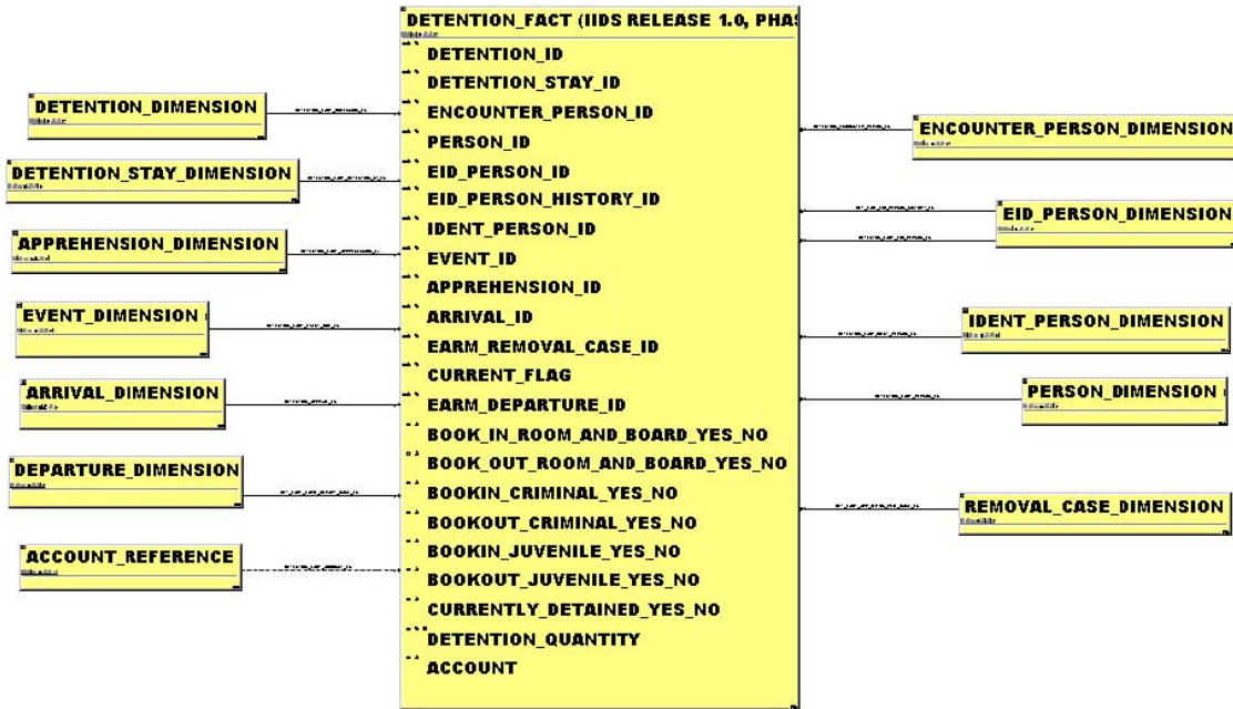
Figure 4. Detention Dimensional Model
