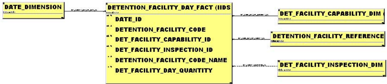
Figure 7. Detention Facility Day Dimensional Model
