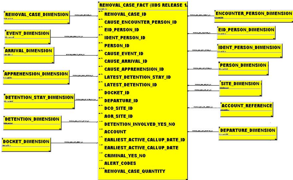
Figure 9. Removal Case Dimensional Model
