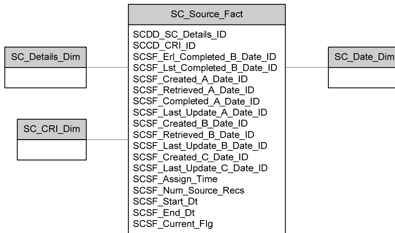
Figure 11. Secure Communities Dimensional Model
