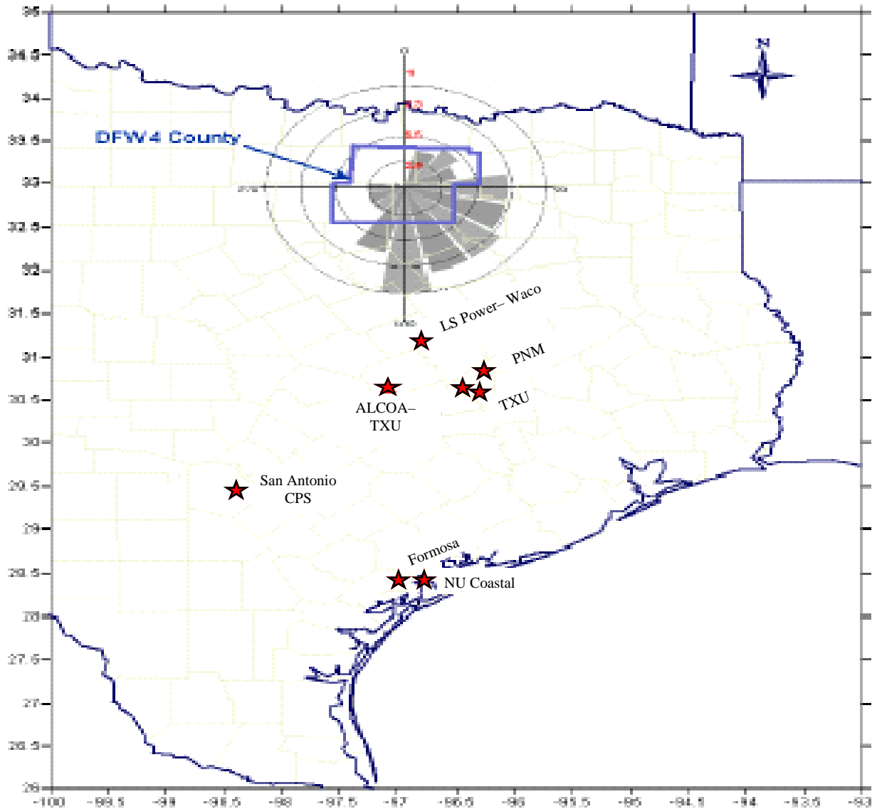
The Wind Rose depicts the frequency of net transport daily winds for 1-hour ozone greater than 125 ppb. The Wind Rose is centered over the D/FW region and includes all sites for the calculation.
